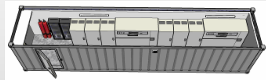
Service Container
